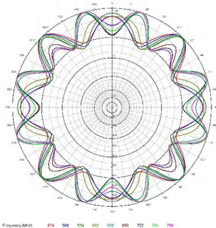
Horizontal radiation pattern with a cross section of 800 mm
